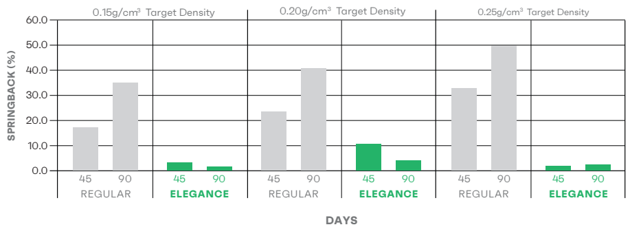
At various target densities, Elegance shows significantly improved embossing and lower springback at 45 and 90 days post-compression.
